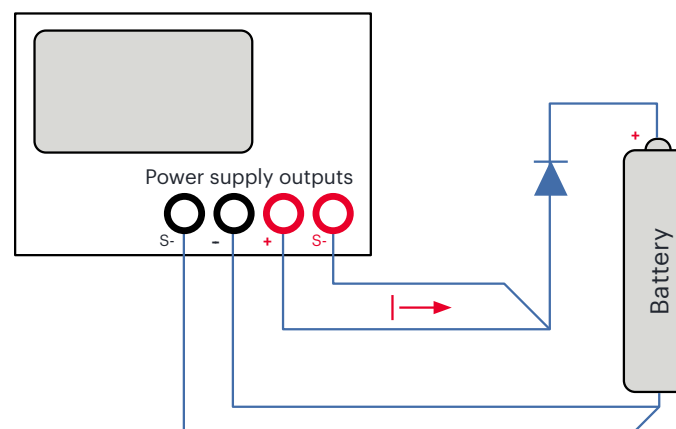
Figure 3. A diode ensures that current flows out of a power supply to a battery and not in the reverse direction.
