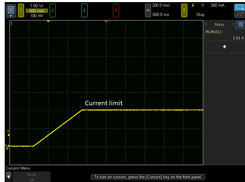
Figure 7. A device using increasingly higher current until the power supply switches to constant current mode
