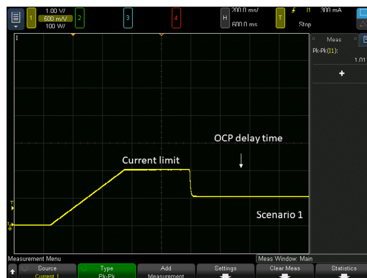
Figure 9. In scenario 1, the power supply returns to constant voltage mode before tripping the delayed OCP
