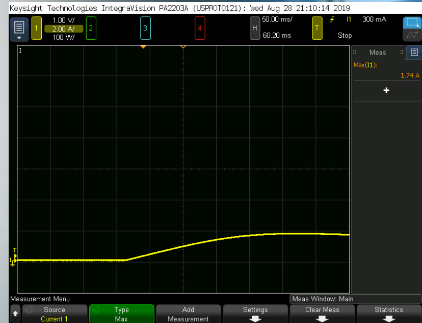
Figure 6. The variable slew rate of 10 V/s eliminates the inrush current
